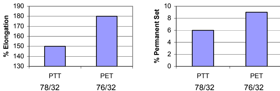
Figure 17: (a) % Elongation performance for fabrics @ 10 N force; (b) % Permanent set for fabrics after elongation @ 10 N force (ref 6)
