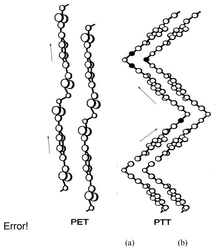
Figure 3: Structural differences between PET and PTT (ref 3)
