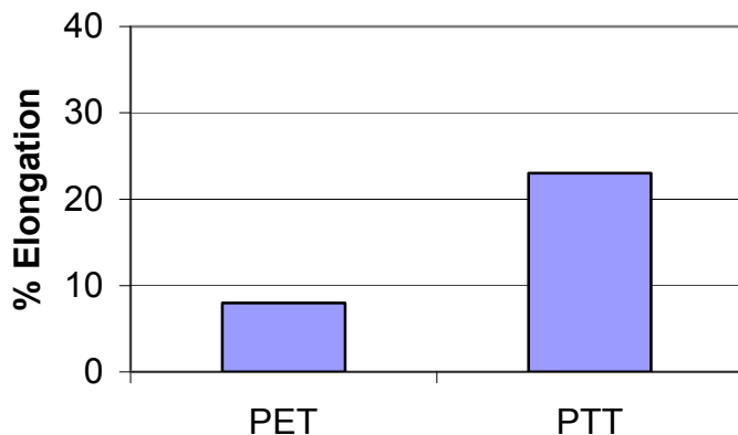
Figure 18: % Elongation in the weft direction of PET and PTT woven fabrics (ref 6)
