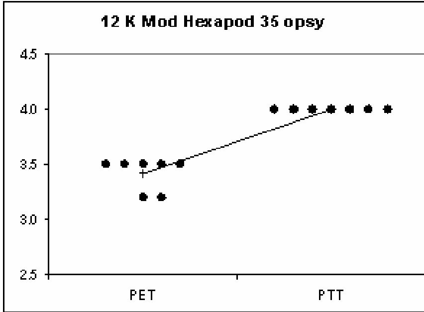
Figure 15(b) : Hexapod Wear Test – 35-Oz Per SqYd (opsy) carpet, 12K cycles
