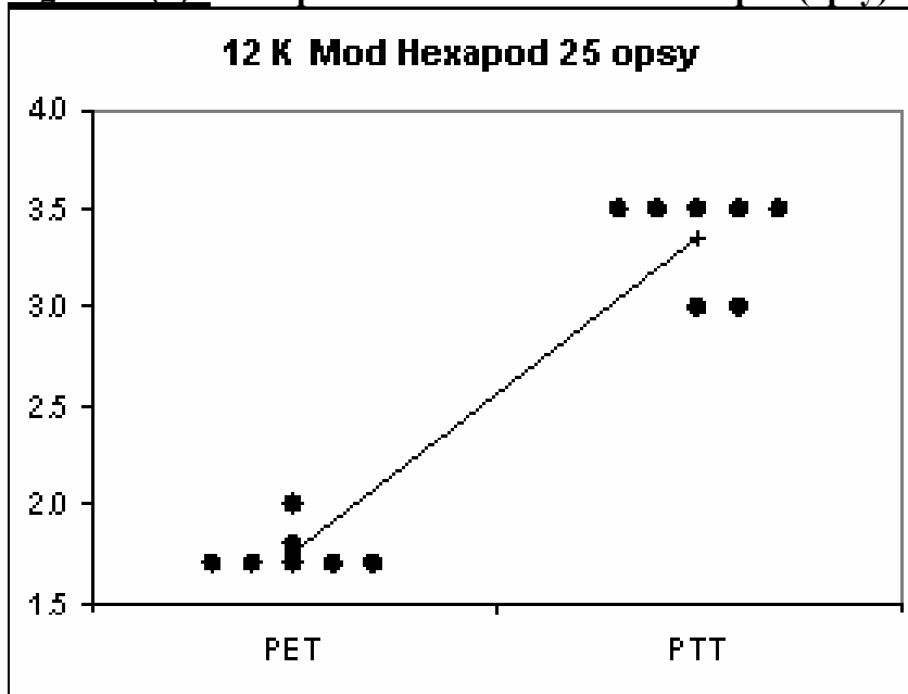
Figure 15(a) : Hexapod Wear Test – 25 Oz Per SqYd (opsy) carpet, 12K cycles
