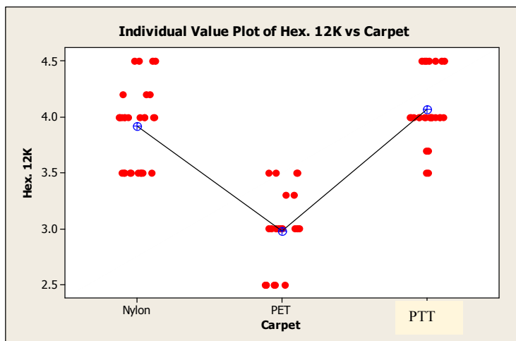
Figure 9: Hexapod Wear Test (12K Cycles)
